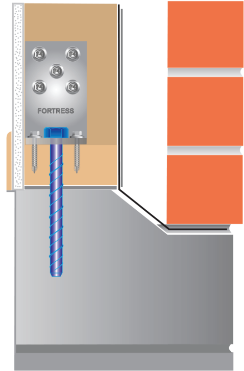
BRACED EXTERNAL FRAME CROSS SECTION
